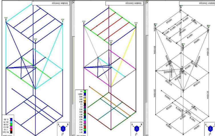
3-D Frame Analysis in Seismic Zone
